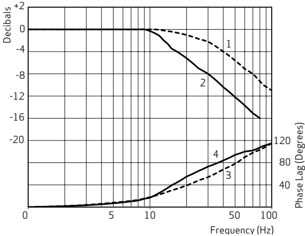
High Frequency Response
