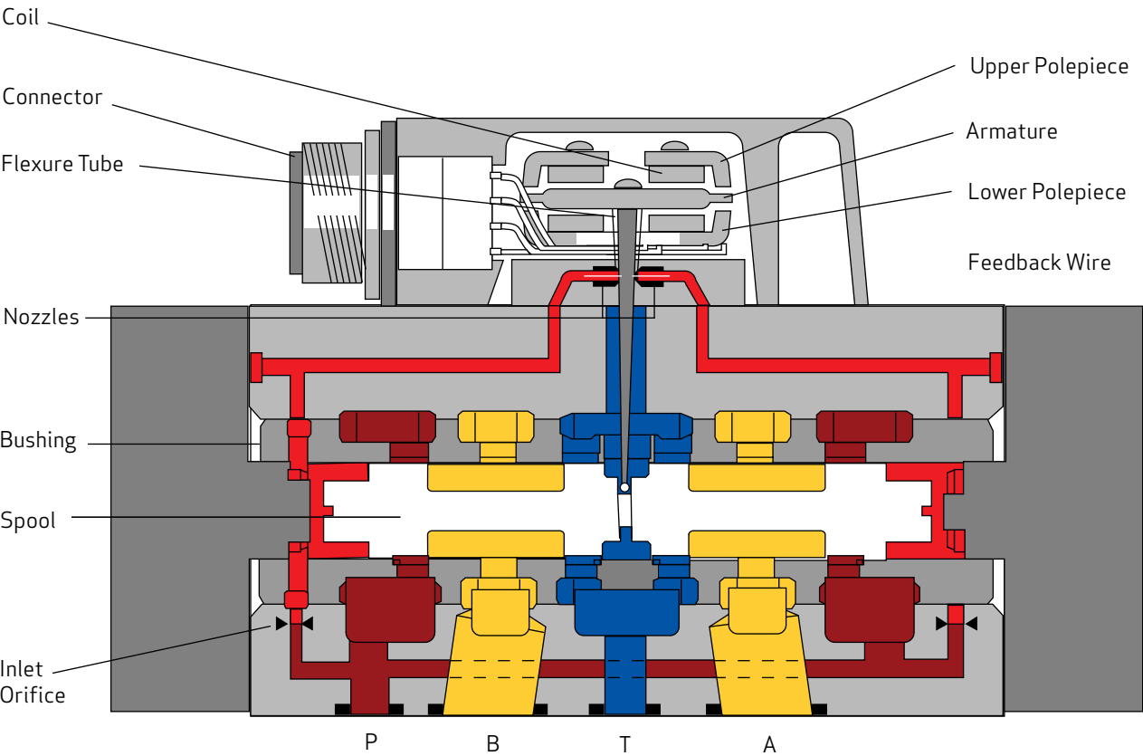
Electro-hydraulic Servo Valve Cut-away
