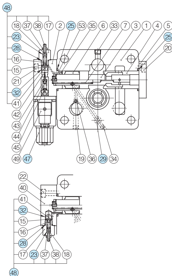
Without Proportional Pilot Relief Valve
