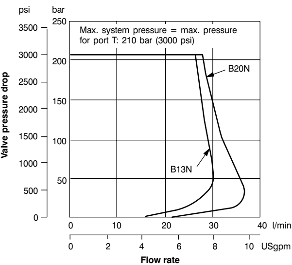
K(A)TG4V-3 Parallel Flow Path
