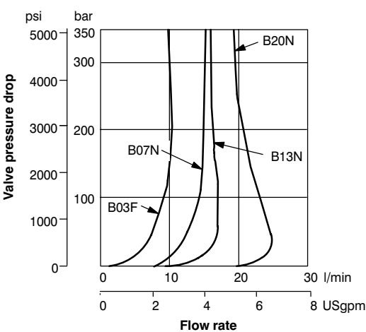
K(A)TG4V-3 Single Flow Path
