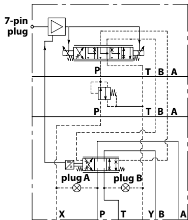
Detailed Symbol
